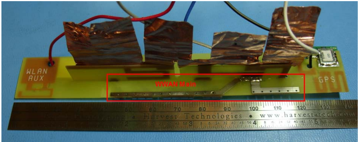
Figure 6 Armor X7 Antenna Assembly Back
